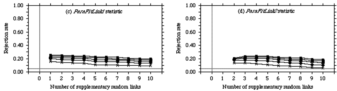
Type I error of test of a supplementary random link
