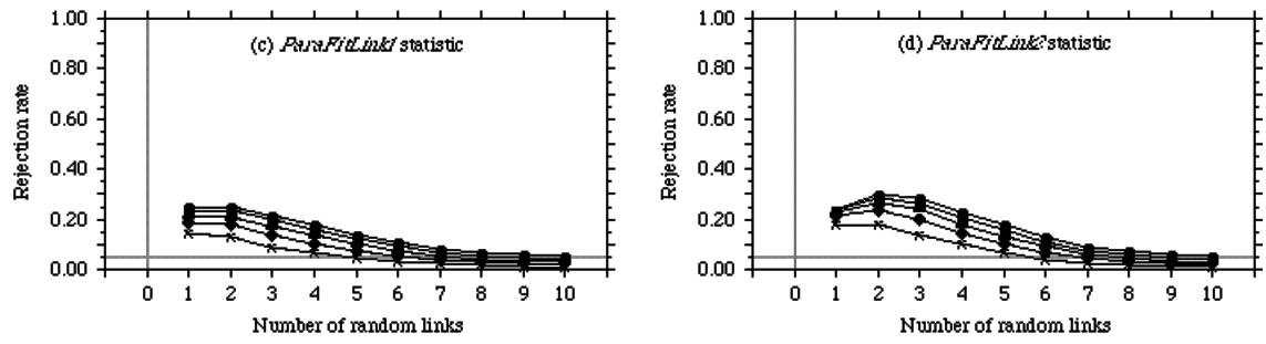
Type I error of test of a random link replacing a coevolutionary link
